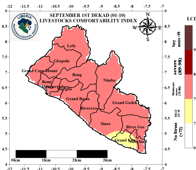
Figure 10: First dekad Livestock LCI
