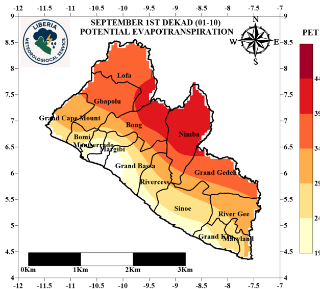
Figure 9: First dekad PET
