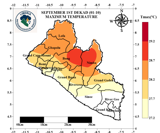
Figure 5: Maximum temperatures at 2m
